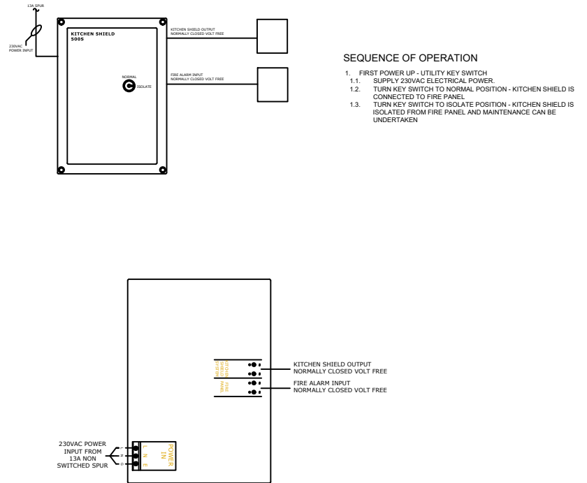
① DETAIL - KITCHEN SHIELD 500S N.T.S.
